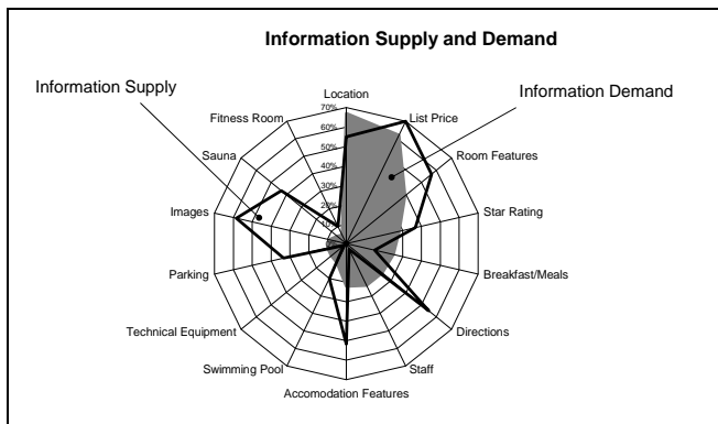
Figure 5. Information supply and demand for available WWW resources
